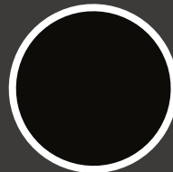
NEW MOON
