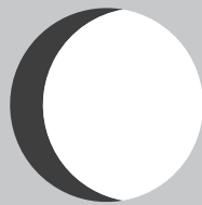
WAXING GIBBOUS
