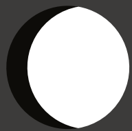
WAXING GIBBOUS
