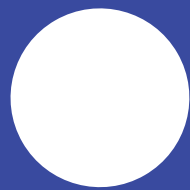
FULL MOON
