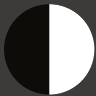
FIRST QUARTER
