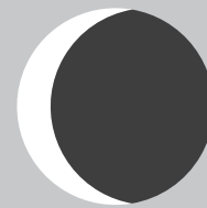
WANING CRESCENT
