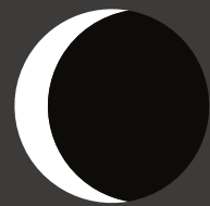
WANING CRESCENT
