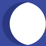
WAXING GIBBOUS
