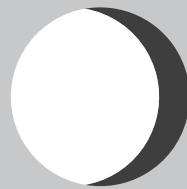
WANING GIBBOUS
