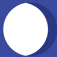
WANING GIBBOUS
